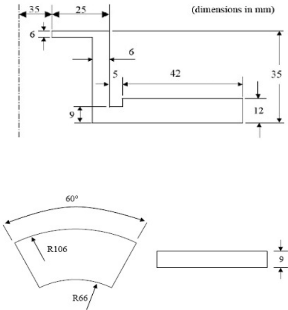
Fig2.the model of disk and pad, and simulation data used in the FE analysis
