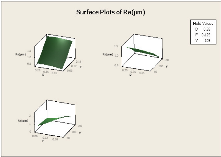
Fig5.Surface Plots for surface roughness (Ra)
