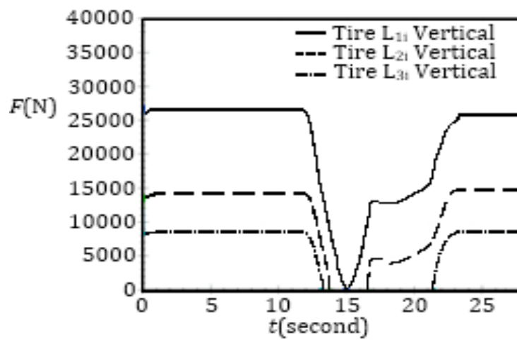
Figure 7: In turn tires vertical forces while rollover
