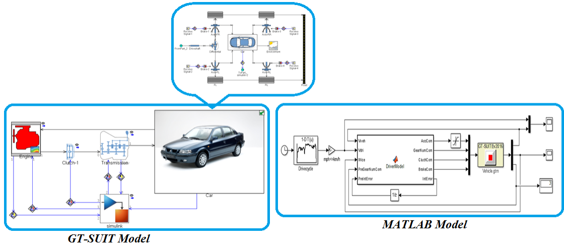
Figure 2. Hybrid simulation of Samand LX vehicle in GT-SUIT and MATLAB
