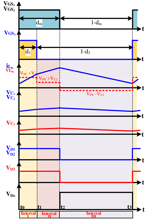
Figure 4: Typical waveforms of the components.
