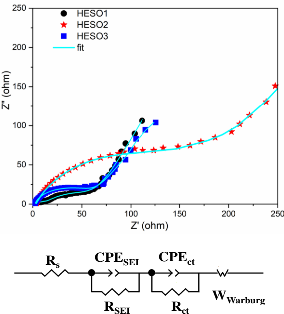
Figure 5: Nyquist plots of HESOs.
