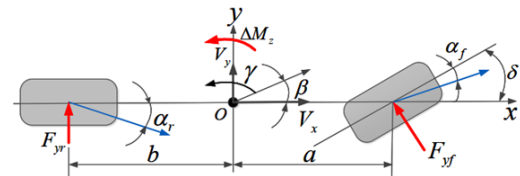
Figure 1: 2-DOF Vehicle dynamics model
