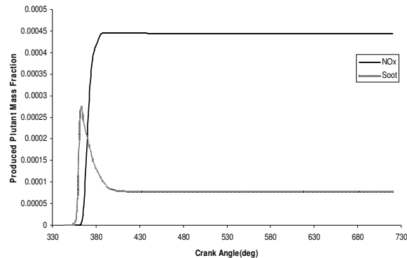
Fig10. NO x and Soot Mass Fraction-Crank Angle Diagram
