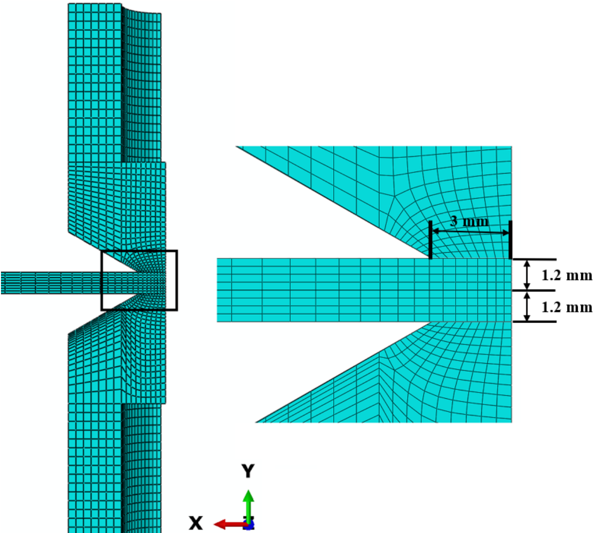
Fig. 2. The finite element model geometry and mesh.
