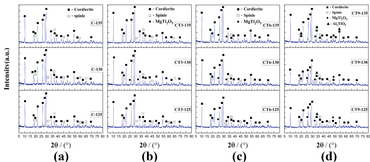
Fig. 2. XRD analysis of cordierite samples at different temperatures (1250°C, 1300°C, and 1350°C): a) Cordierite (C-125, C-130, and C135), b) Cordierite with 3 wt.% of TiO 2 (CT3-125, CT3-130, and C T3-135), c) Cordierite with 6 wt.% of TiO 2 (CT6-125, CT6-130, and C T6-135), and d) Cordierite with 9 wt.% of TiO 2 (CT9-125, CT9-130, and C T9-135)
