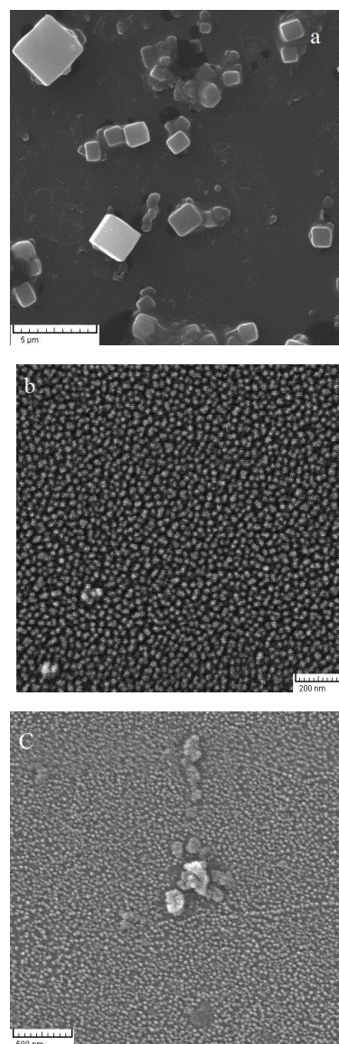
Fig. 5. SEM micrographs of starting materials as well as prepared \text{MgAl}_2\text{O}_4 powder by molten salt method at 850 °C for 3h. (a) magnesia, (b) \gamma -alumina from boehmite precursor, and (c) synthesized spinel.
