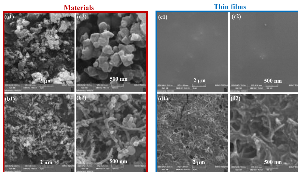
Fig. 8. Fig. 8. Scan electron microscopy (SEM) images of (a1) poly2-Aminobenzothiazole, (b1) poly 2-aminobenzothiazole: MWCNTs composite, (c1) poly 2-Aminobenzothiazole thin film, and (d1) poly 2-aminobenzothiazole: MWCNTs composite thin film.
