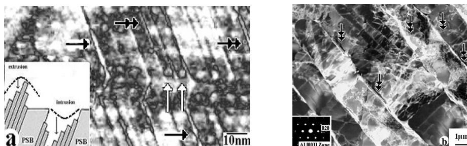
Fig. 7. Microstructures of the necked regions of dendrites arms, similar to the boxed area of Fig. 3(d): AFM of slip lines, and (b) TEM image of slip lines and Selected Area Diffraction Patterns.
