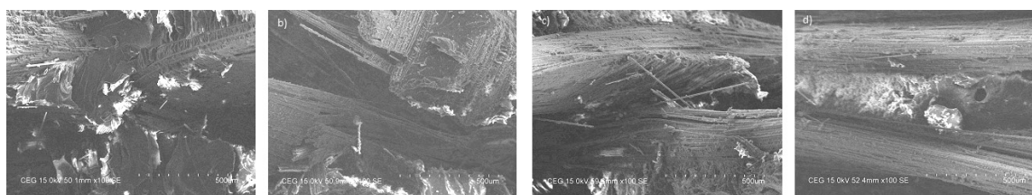
Fig. 4. SEM image a) neat, b) 0.2wt%, c) 0.5wt% and d) 1wt% of CNF in biaxial carbon fibre composites respectively.
