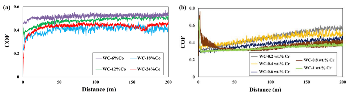
Fig. 11. COF-distance diagrams of the studied cermets: a) WC-Co and b) WC-Cr
