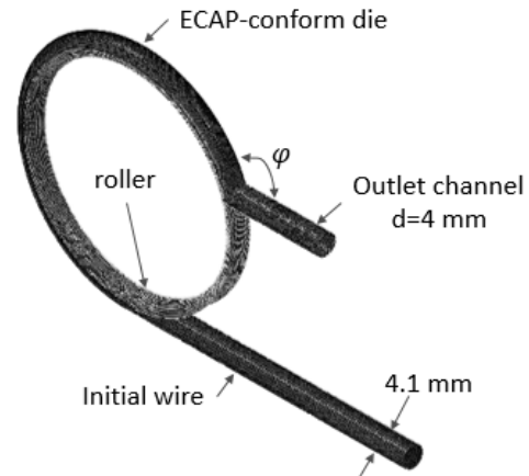
Fig. 2. FE model
