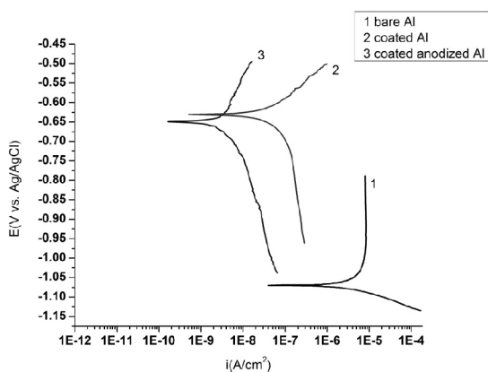
Fig. 5. Tafel plot for bare and coated aluminum. (1) bare Al. (2) coated Al. (3) coated anodized Al.
