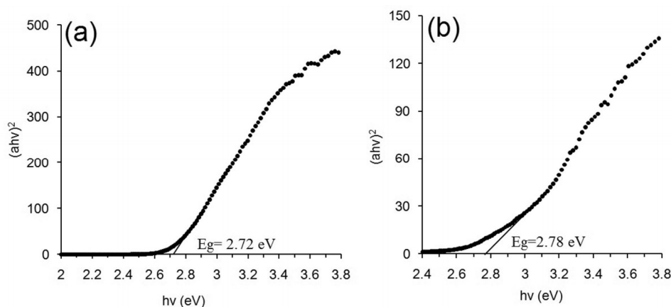
Fig. 5. The plots of (\alpha h\nu)^2 vs. h\nu (eV) for \text{Ag}_6\text{Mo}_{10}\text{O}_{33} (a) and Ni-substituted product (b).
