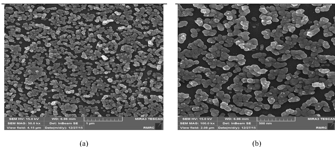
Fig. 12. The SEM micrographs of as-quenched 65\text{GeO}_2\text{-}15\text{PbO}\text{-}10\text{MgO}\text{-}10\text{MgF}_2 sample after annealing at 700^\circ\text{C} for 30 min, a) complex overview; b) more detailed view.
