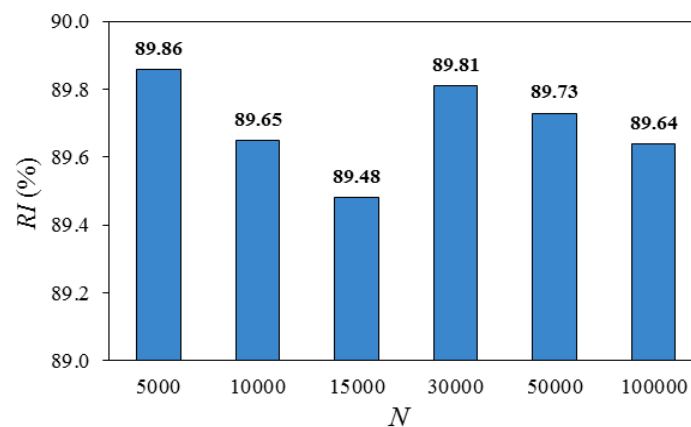
Figure 3. Results of sensitivity analysis for the first topology optimization case
