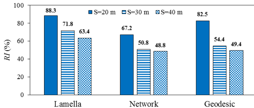
Figure 6. Reliability index of optimal domes for Q = 250 \text{ kg/cm}^2
