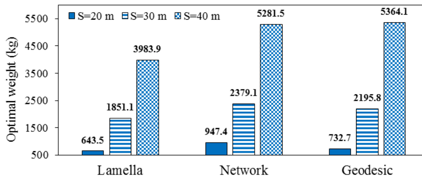
Figure 5. Optimal weight of domes for Q = 375 \text{ kg/cm}^2
