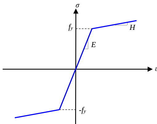
Figure 2. Material constitutive behavior of steel
