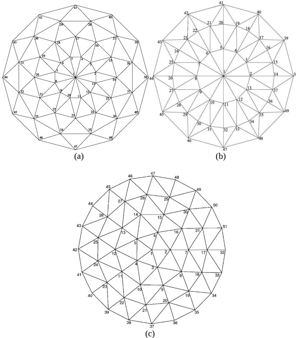
Figure 1. Plan view of (a) Lamella, (b) Network and (c) Geodesic lattice domes
