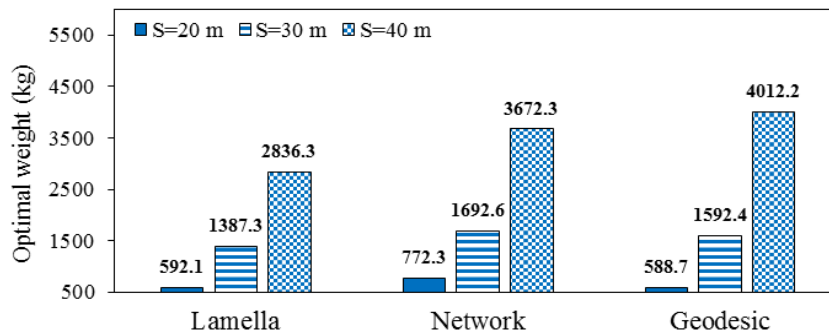
Figure 4. Optimal weight of domes for Q = 250 \text{ kg/cm}^2
