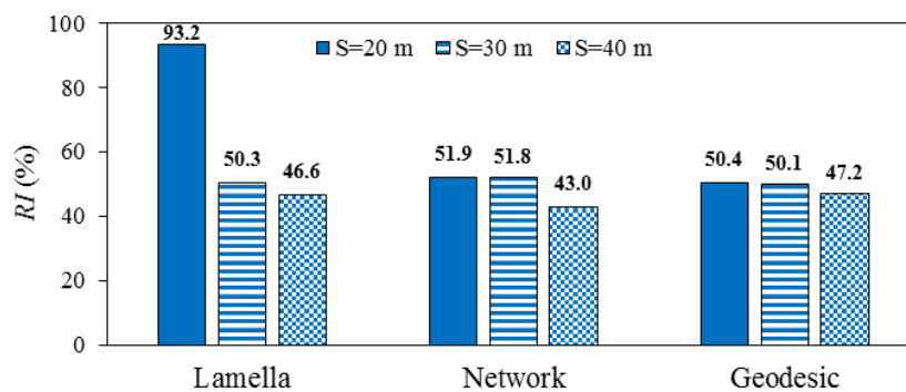
Figure 7. Reliability index of optimal domes for Q = 375 \text{ kg/cm}^2
