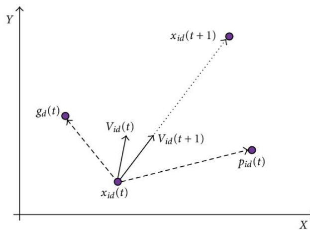
Figure 4. Moving a particle in PSO
