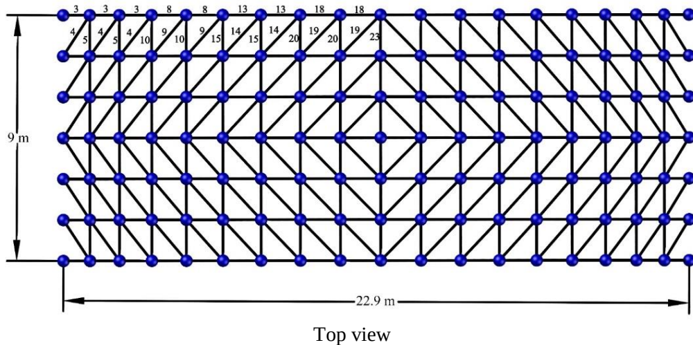
Figure 6. The 693-bar double-layer barrel vault
