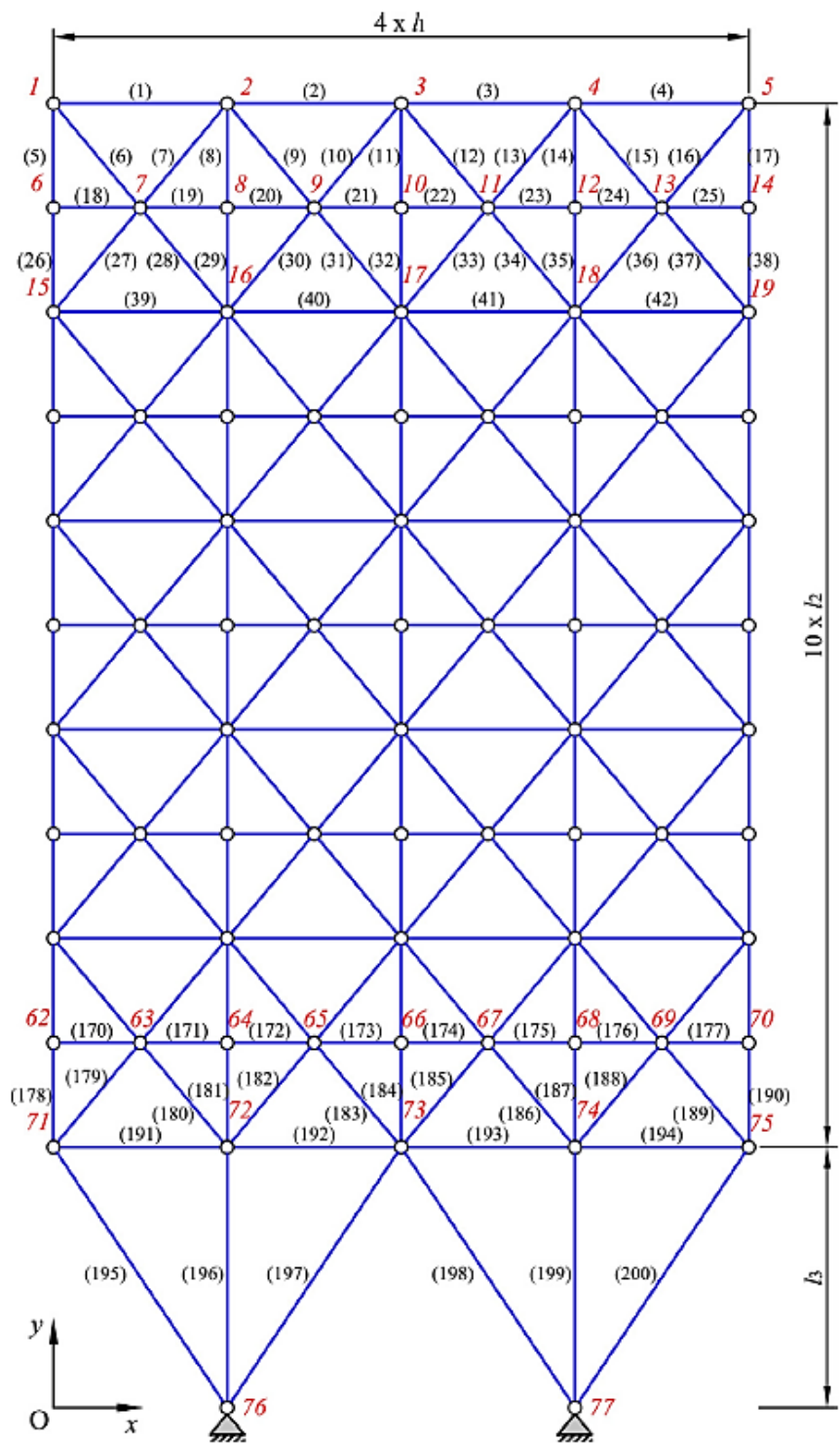
Figure 6. 200-bar truss
