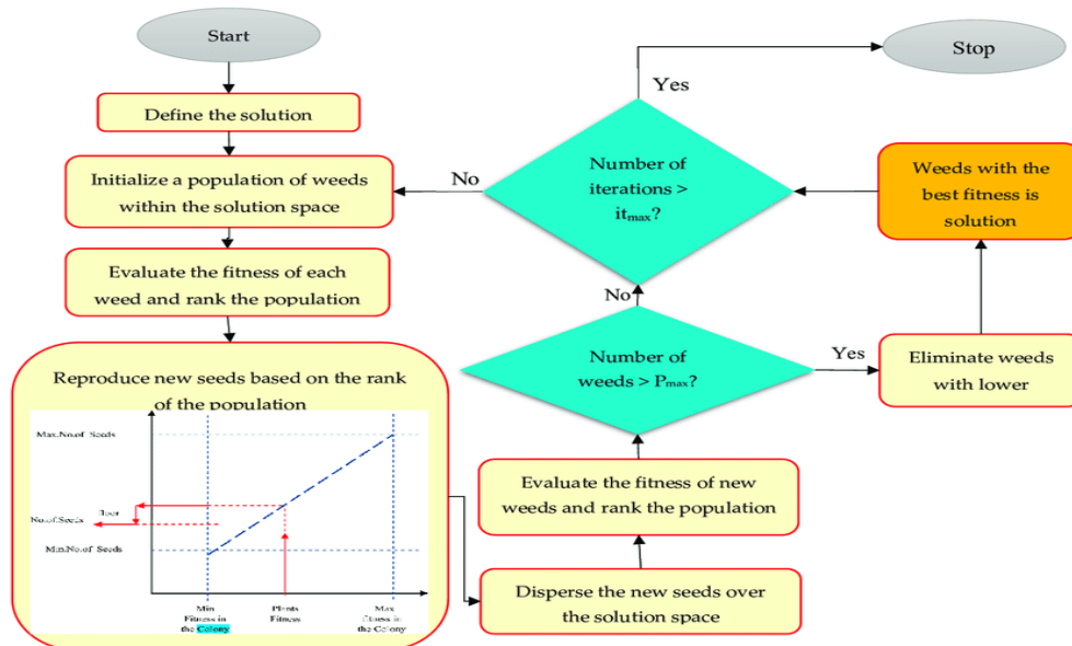
Figure 1. Weed Algorithm Flowchart [21]
