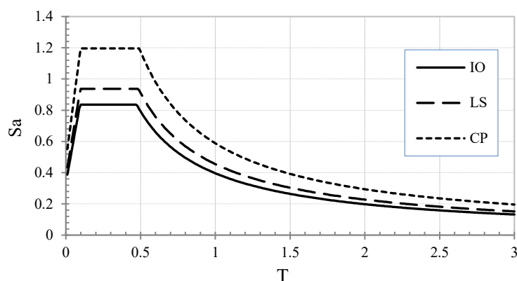
Figure 1: Response spectrum curve
