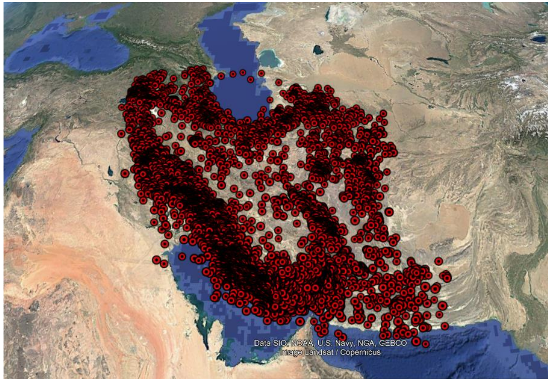
Figure 5: Predicted earthquakes 1900-1963
